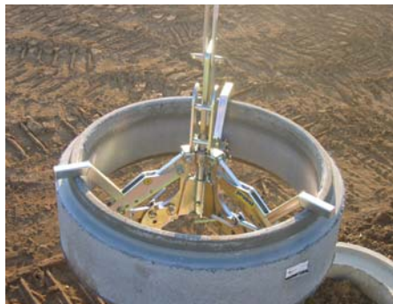
Manhole rings with inner diameters from 625 to 1500 mm are installed safely and accurate to the millimeter.
